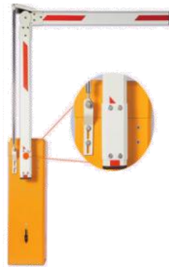
90° Folding Arm
